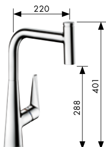
Talis® Select S 300 Single lever kitchen mixer with pull-out spout, swivel range 150° #72821,-000,-800
