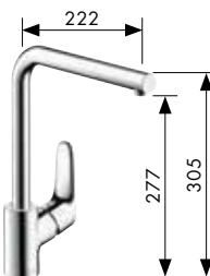
Focus® 280 Single lever kitchen mixer with swivel spout 110°/150°/360° # 31817,-000
