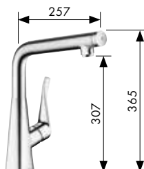
Metris® Select 320 Single lever kitchen mixer with swivel spout 110°/150°/360° #14883,-000,-800
