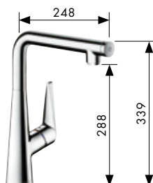
Talis® Select S 300 Single lever kitchen mixer with swivel spout 110°/150°/360° #72820,-000,-800
