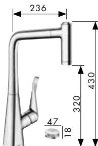
M7120-H320 2-hole single lever kitchen mixer with pull-out spray and 2 spray types #73806,-000,-800
