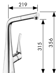
Metris® 320 Single lever kitchen mixer with pull-out spout 110°/150°/360° # 14821,-000,-800
