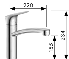
Logis® 160 Single lever kitchen mixer with swivel spout 360° # 71832,-000 # 71833,-000 for installation in front of a window (not shown) # 71834,-000 with shut-off valve (not shown) # 71839,-000 CoolStart Eco (not shown)
