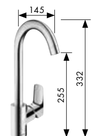
Logis® 260 Single lever kitchen mixer with swivel spout 110°/150°/360° # 71835,-000
