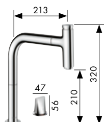
M7119-H200 2-hole single lever kitchen mixer with pull-out spout, swivel range 150° #73804,-000,-800
