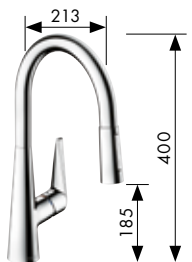
Talis® S 200 Single lever kitchen mixer with pull-out spray, two spray types, swivel spout 110°/150° # 72813,-000,-800
