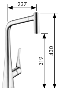
Metris® 320 Single lever kitchen mixer with pull-out spray, two spray types, swivel spout 110°/150° # 14820,-000,-800
