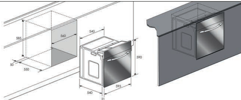
INSET HOLE TECHNICAL DRAWING VALID FOR ALL ELLECI OVENS
