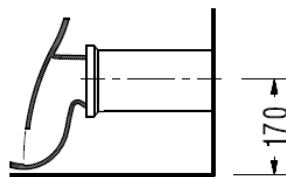
P-trap installation
